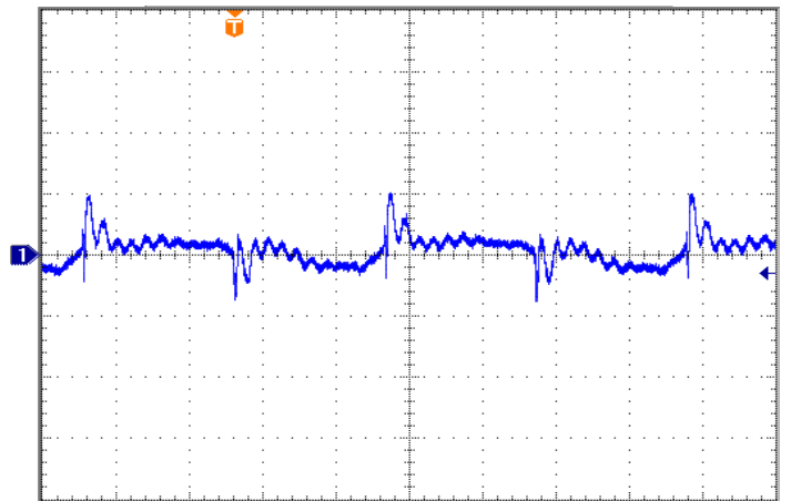
Figure 16: Output Ripple voltage at nominal input voltage and rated load current (100 mV/div, 2 \mu s/div). Load capacitance: one 1.0 \mu F ceramic capacitor and one 15 \mu F tantalum capacitor. Bandwidth: 20 MHz. (See Figure 13).
